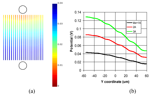
Figure 6. (a) Potential distribution in source net (metal 1 layer) and (b) its 1D cross-section in the leftmost metal line for different current levels (enabling current sense point design).
